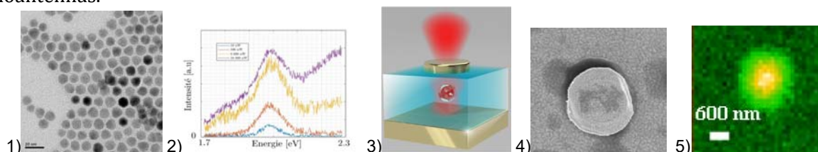
Figure: 1) TEM images of CdSe/CdS nanocrystals 2) CdSe/CdS spectra broadening under increasing excitation 3) patch antenna 4) SEM image of patch antenna 5) emission pattern of patch antenna
